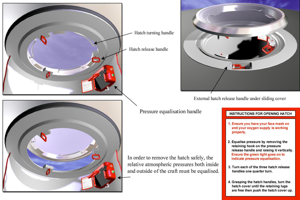
IGV Top Emergency Escape/Access Hatch - Fig. II
