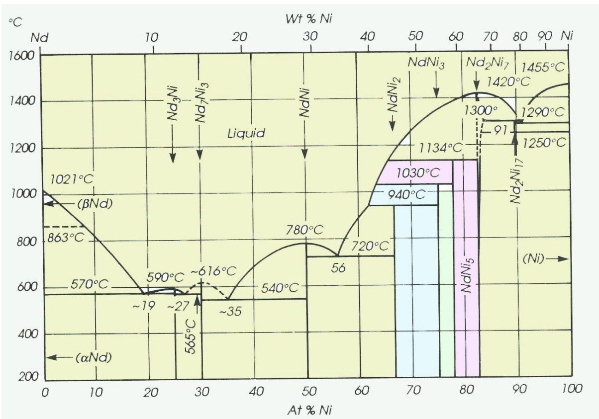
This is the equilibrium diagram of Neodymium Nd-60 with 1% of Nickel Ni-28.
