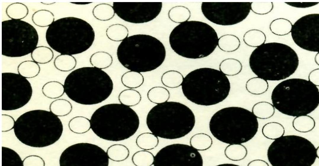
Figure 13-1. Water magnified one billion times.
